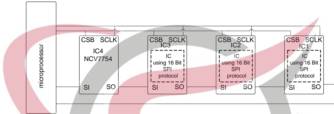
Figure 31. Serial Daisy Chain
